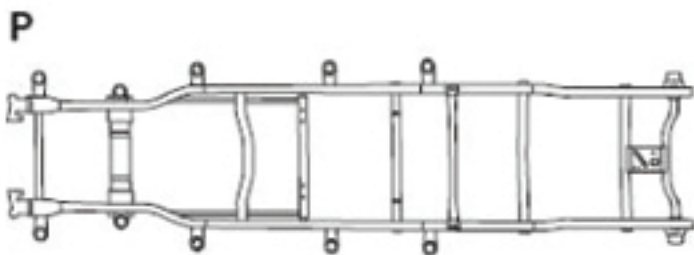
UNDERBODY VIEW
